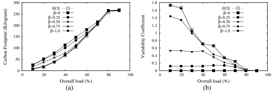
Fig. 3. Total carbon footprint (a) and variability coefficient (b) vs. the overall load with different values of the parameter \beta .
