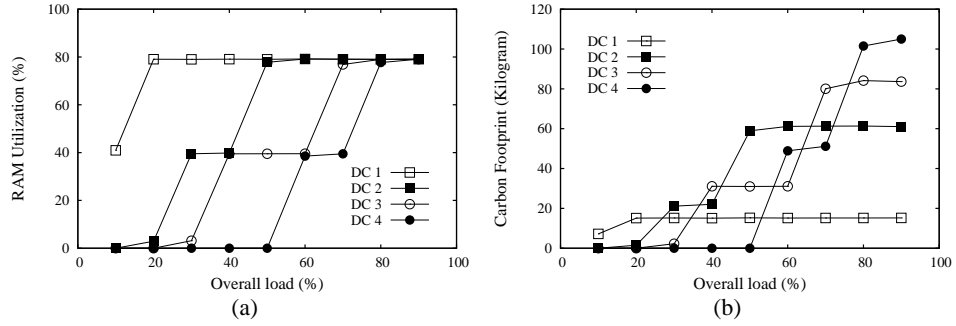
Fig. 6. RAM utilization (a) and carbon footprint (b) of the four data centers vs. the overall load with \beta=1 .
